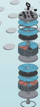
FILTER PACK WITH HIGH PROFILE DISCS
